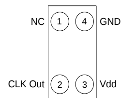
Figure 1. Pin Assignment
