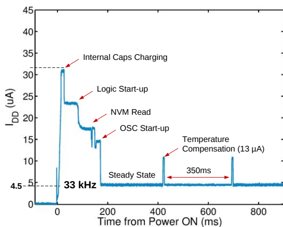
Figure 5. Start-up and Steady-State Current Profile
