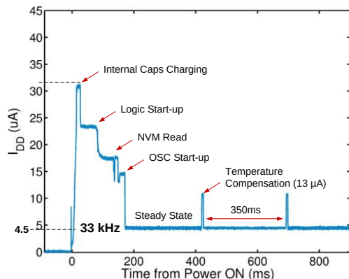
Figure 8. Start-up and Steady-State Current Profile
