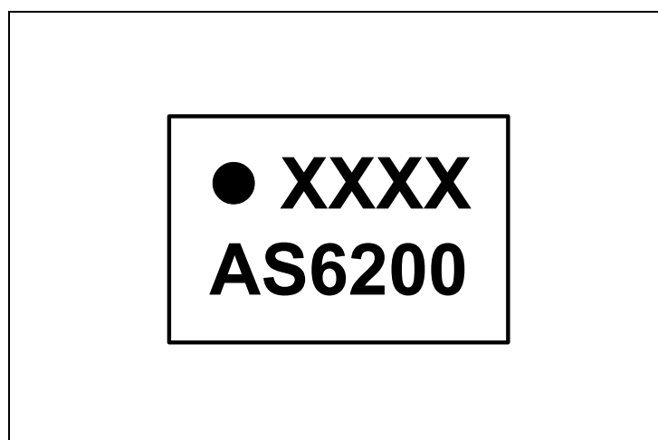
Figure 40: Package Code
